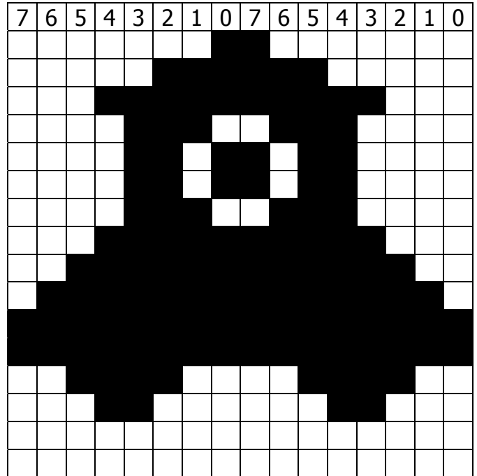
16*16 sprite representation
