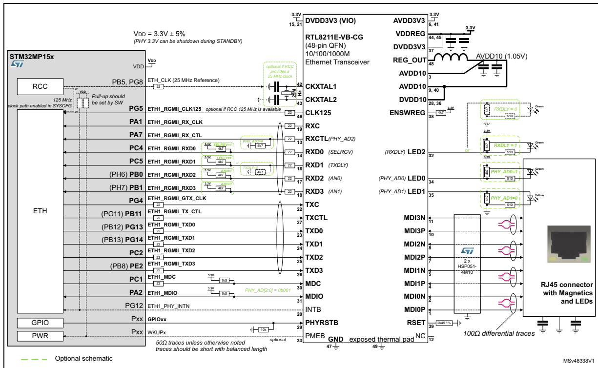
Figure 46. Gigabit Ethernet PHY connection example with V_{DD} = 3.3\text{ V} (RTL8211E)
