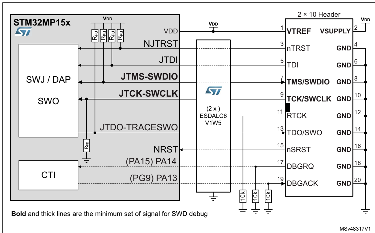
Figure 18. JTAG/SWD MIP110 connector implementation example
